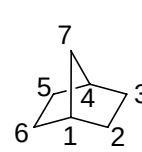
降冰片烷
